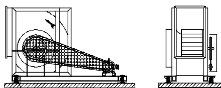
SPRING ISOLATOR
