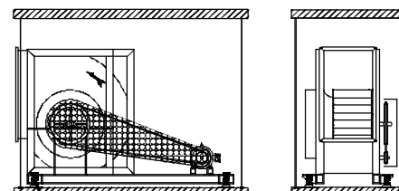
SPRING ISOLATOR
