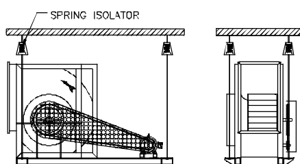
CEILING-MOUNT HANGER TYPE
